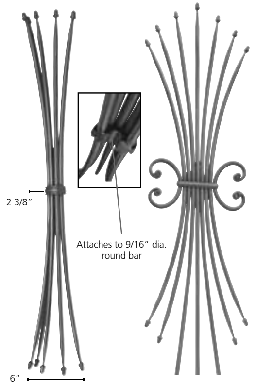
Art. GD253/1 Mtl 1/2" dia. W 6" H 39 3/8" Wt. 8.2 lbs.
