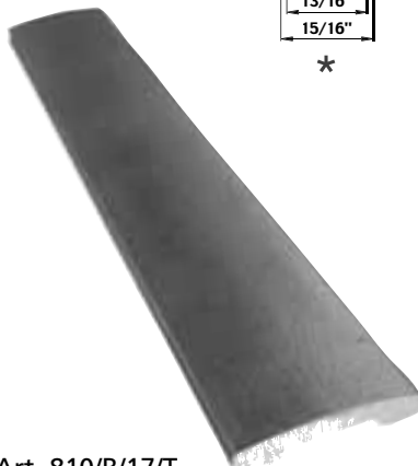
Art. 810/B/17/T L ≈ 19' 8" approx. Wt. 37.8 lbs.
