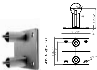
AISI 304 AISI 316 For tube A E401/304 E401 1 2/3" dia. x 5/64"
