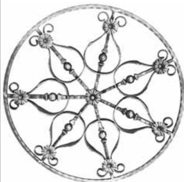
Art. 718/1 Mtl 9/16" sq. 28 15/16" dia. Wt. 28.6 lbs.
