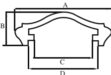
Art. 811/5/ALL A 2 1/8" B 3/4" C 1 9/32" D 1 17/32" Wt. 9.94 lbs. L 20' approx.
