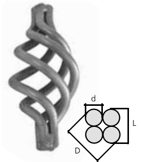
4 Round filaments Art. 1163/3 d 1/4" D 37/64" L 1/2" x 4 15/16" Wt. 0.4 lbs. Art. 1163/4 d 9/32" D 21/32" L 9/16" x 4 15/16" Wt. 0.5 lbs.
