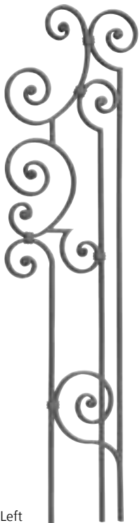
Art. GD163/2 Mtl 9/16" x 5/16" 11 1/32" W x 39 3/8" H Wt. 10.3 lbs.
