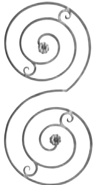
Art. 1038/1/ALL Mtl 9/16" sq. W 20 5/64" H 42 33/64" Wt. 7.7 lbs
