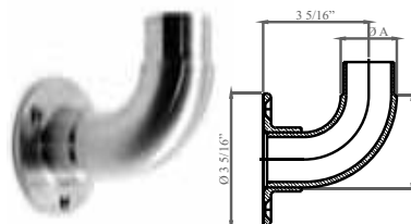
AISI 316 For tube A E4561 1 2/3" dia. x 5/64"
