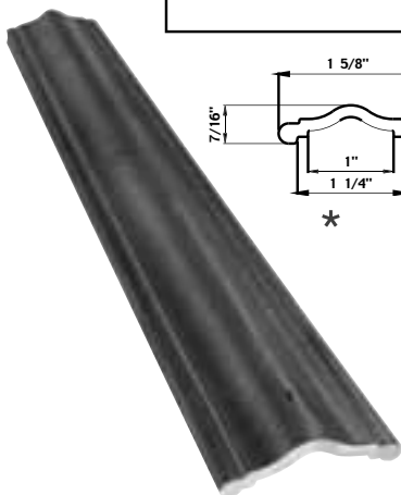
Art. 811/7/T L ≈ 19' 8" approx. Wt. 20.7 lbs.
