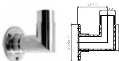
AISI 316 For tube A E4566 1 2/3" dia. x 5/64"
