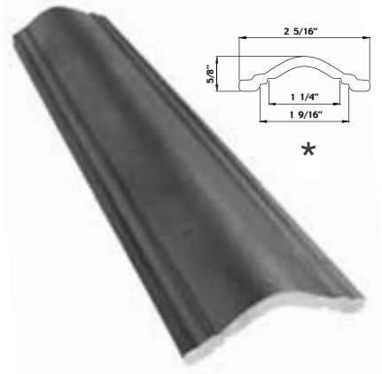
Art. 811/6/T L ≈ 19' 8" approx. Wt. 36.1 lbs.
