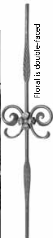
Art. 1135/1 Mtl 9/16" dia. W 8 5/8" H 39 3/8" Wt. 4.4 lbs.
