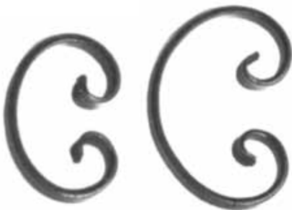
Art. 80/A/9 Mtl 1/2" x 1/4" W 2 3/4" x H 4 1/8" Wt. 0.35 lbs.
