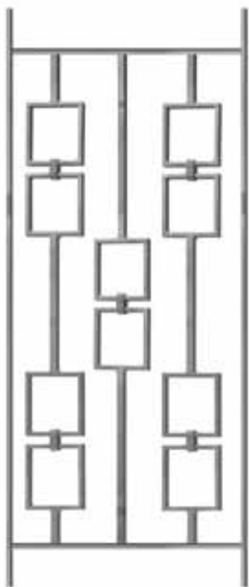
Art. GD183/1 Mtl 9/16" x 5/16" sq. W 15 3/4" x H 39 3/8" Wt. 17.38 lbs.
