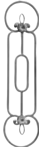
Art. 1685/1 (ex 9133/1) Mtl 9/16" sq. H 39 3/8" Wt. 13.6 lbs.
