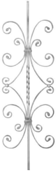
Art. 769/6 Mtl 9/16" sq. W 11 13/16" H 35 7/16" Wt. 3.3 lbs.
