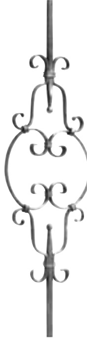
Art. 64/A/2 Mtl 1/2" sq. W 10 1/4" H 35 7/16" Wt. 5.0 lbs.
