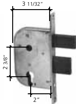
Art. 181/12 W 4 1/8" H 11 1/4" Wt. 1.8 lbs.
