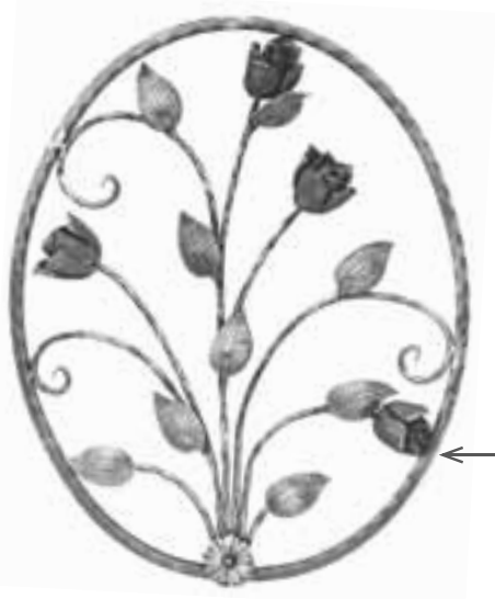
Art. 720/1 Mtl 9/16" W 20 1/4" x H 26 3/8" Wt. 15.4 lbs.
