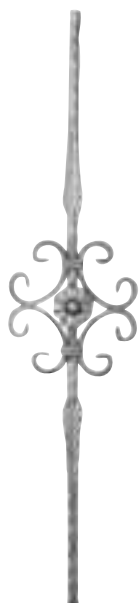
Art. 768/9 Mtl 9/16"sq. W 8 1/4" H 39 1/2" Wt. 1.6 lbs.
