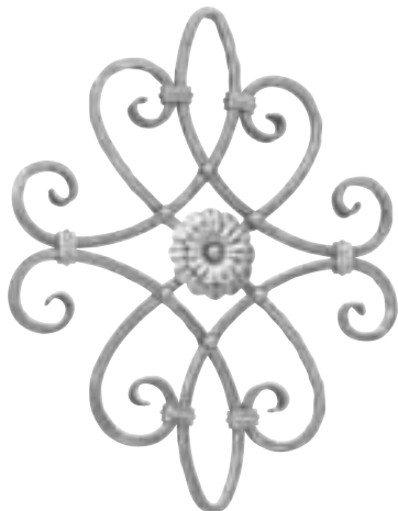
Art. 26/C/1/ALL Mtl. 9/16" sq. W 17" x H 20 1/2" Plain square bar Floral element on one side only Wt. 3.3 lbs.
