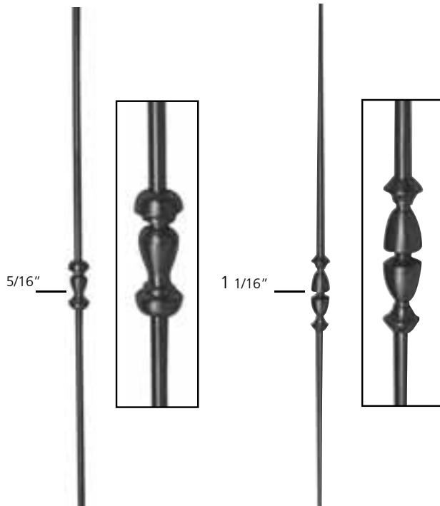
Art. GD251/3 Mtl 1/2" dia. H 39 3/8" Wt. 2.6 lbs.
