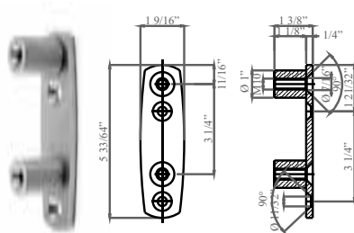
AISI 304 Dimensions E112 5 33/64" x 1 9/16" x 1 3/8"
