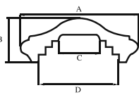
Art. 811/3/ALL A 2 1/4" B 7/8" C 25/32" D 1 17/32" Wt. 17.5 lbs. L 20' approx.
