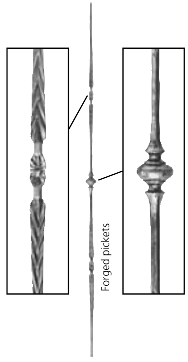
Art. 504/1 Mtl 1/2" dia. H 39 3/8" Wt. 1.9 lbs.
