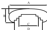
Art. 810/B/15/ALL A 2 1/8" B 3/4" C 1" D 1 17/32" Wt. 20.35 lbs. L 20' approx.
