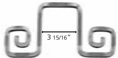
Art. 1145/3 Mtl 1/2" sq. W 12 13/32" x H 6 11/16" Wt. 2.38 lbs.
