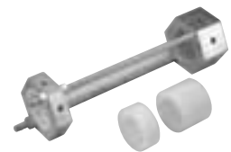
Plastic box containing tool, with M5, M6, M8 mandrels and heads. Riveting tool for threaded inserts M5, M6, M8.
