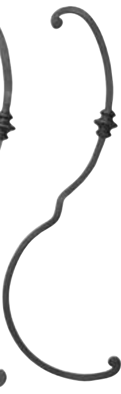
Art. GD0021/Q16 Mtl 5/8" sq. W 11 39/64" approx H 35 53/64" approx Wt. 6.8 lbs.
