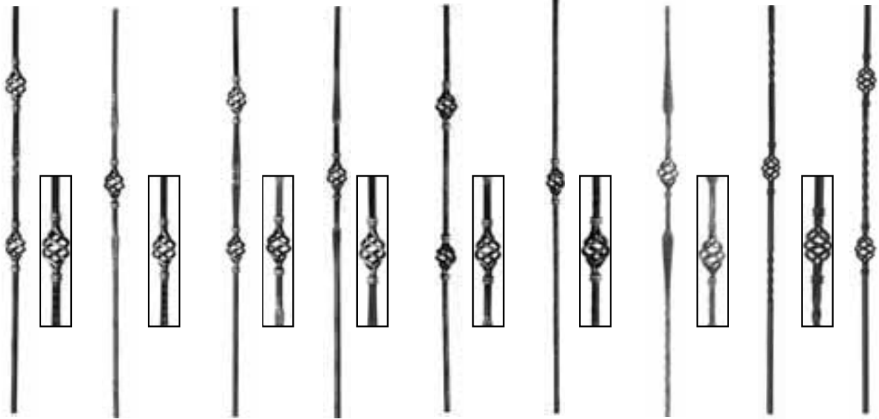
Art. 1158/12 Mtl 1/2" sq. W 2 1/8" H 47" Wt. 4.3 lbs. Art. 1158/13 Mtl 1/2" sq. W 2 1/8" H 47" Wt. 4.3 lbs. Art. 1158/14 Mtl 1/2" sq. W 2 1/8" H 47" Wt. 4.3 lbs. Art. 1158/15 Mtl 1/2" sq. W 2 1/8" H 47" Wt. 4.1 lbs. Art. 1158/16 Mtl 1/2" sq. W 2 1/8" H 47" Wt. 4.3 lbs. Art. 1158/17 Mtl 1/2" sq. W 2 1/8" H 47" Wt. 4.1 lbs. Art. 562/2/L Mtl 9/16" sq. H 47" Wt. 4.4 lbs. Art. 1158/1 Mtl 1/2" sq. W 2 1/8" H 47" Wt. 3.2 lbs. Art. 1158/2 Mtl 1/2" sq. W 2 1/8" H 47" Wt. 3.3 lbs.
