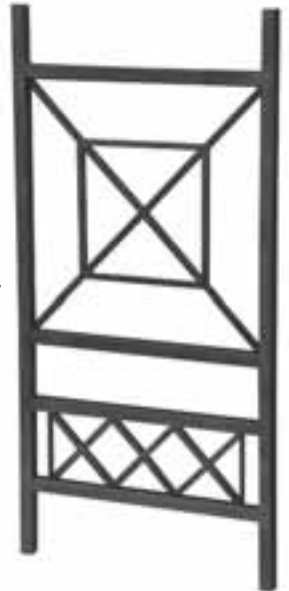
Art. GD76/1 Mtl 1" sq. W 19 11/16" x H 39 3/8" Wt. 23.1 lbs.
