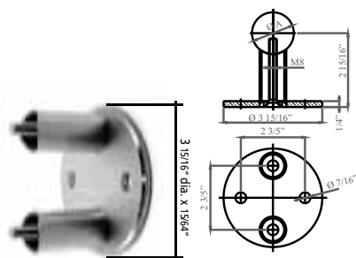
AISI 304 AISI 316 For tube A E400/304 E400 1 2/3" dia. x 5/64"
