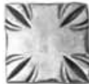
Art. 94/A/3 3 15/16" x 3 15/16" 5/16" Thickn. Wt. 0.8 lbs.
